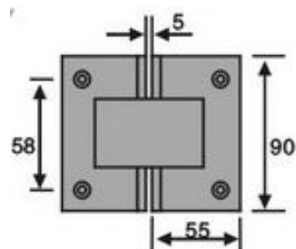
201105-90T 90° S/S Double Glass clamp
